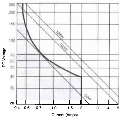
FIGURE 1 - LIMITING CURVE FOR DC POWER LOAD
